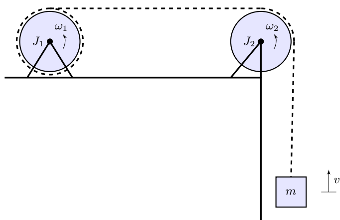
Figure 1: Winch/pulley/mass systems
